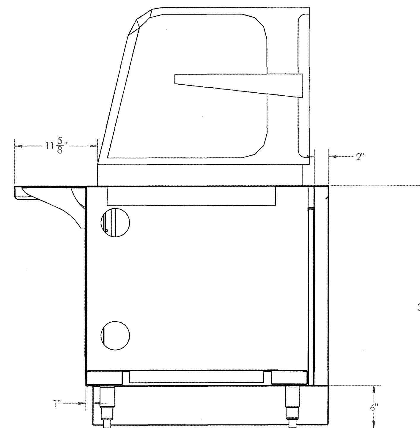
SECTION AT ITEM 3R 1 1/2"=1'-0"
