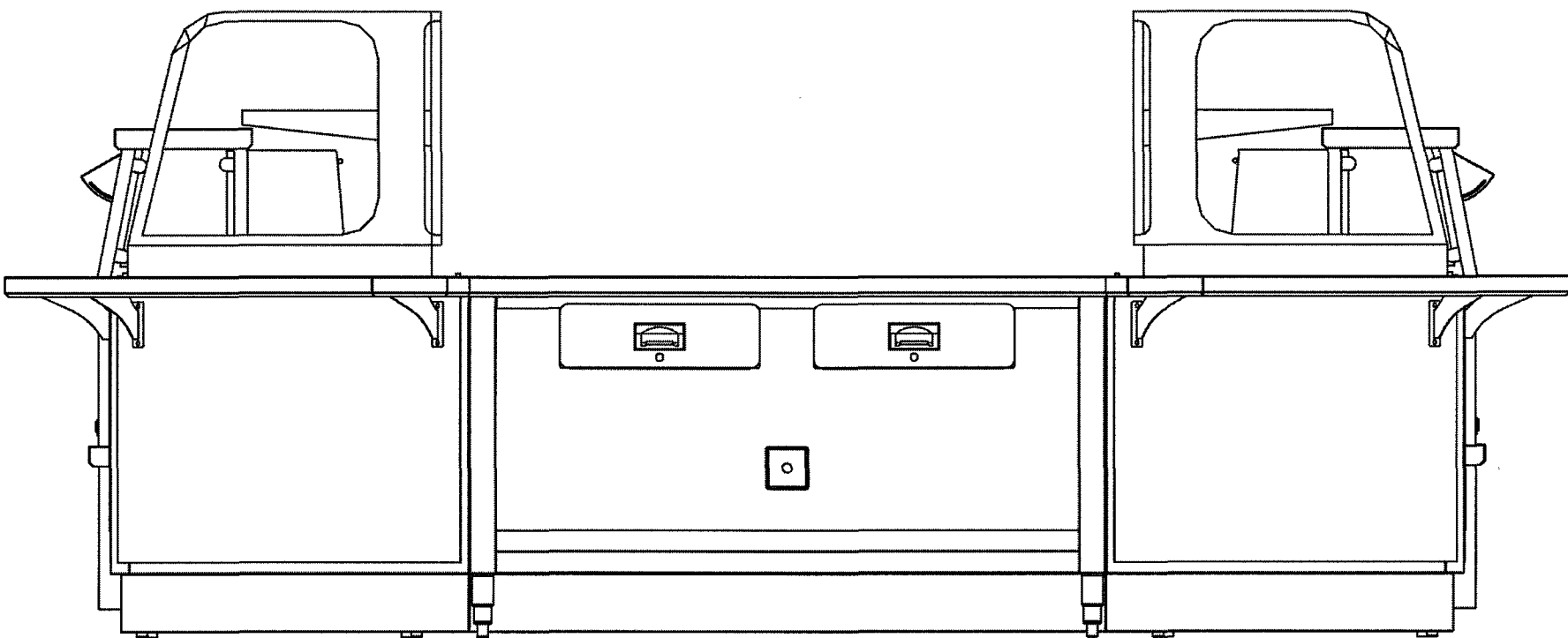
ELEVATION-A AT SERVING LINE
