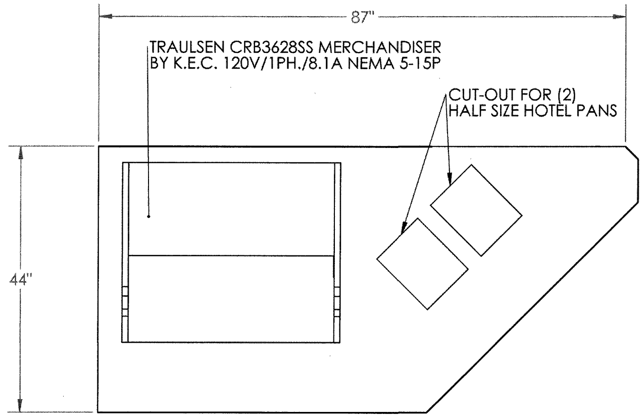
ITEM 3: COLD FOOD COUNTER ONE REQUIRED (1) SCALE 3/4"=1'-0"
