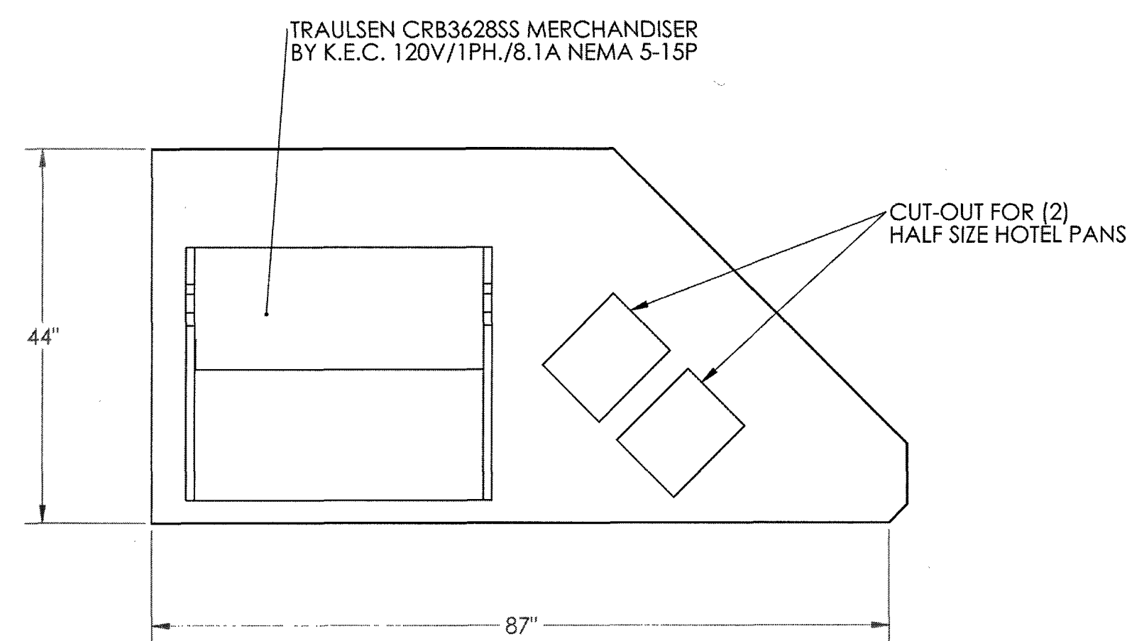
ITEM 3R: COLD FOOD COUNTER ONE REQUIRED (1) SCALE 3/4"=1'-0"
