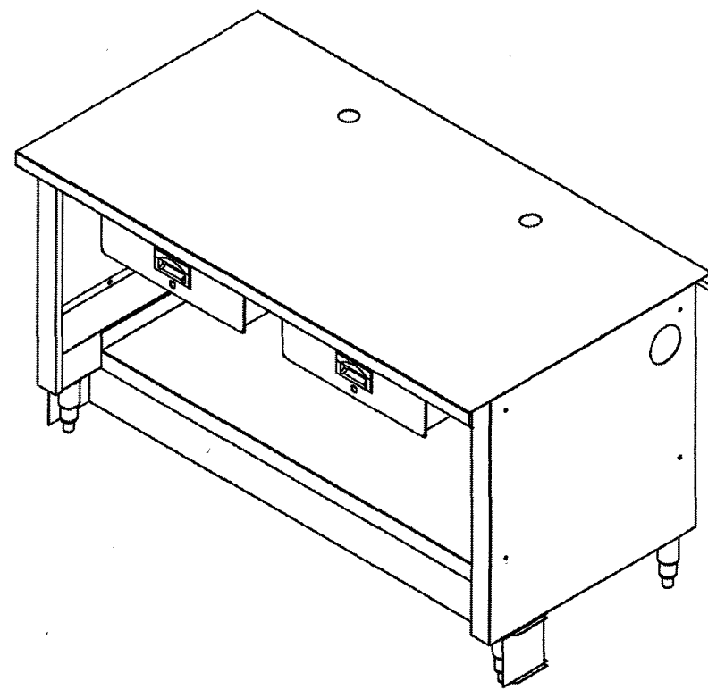
ISOMETRIC-CUSTOMER AT ITEM 4
