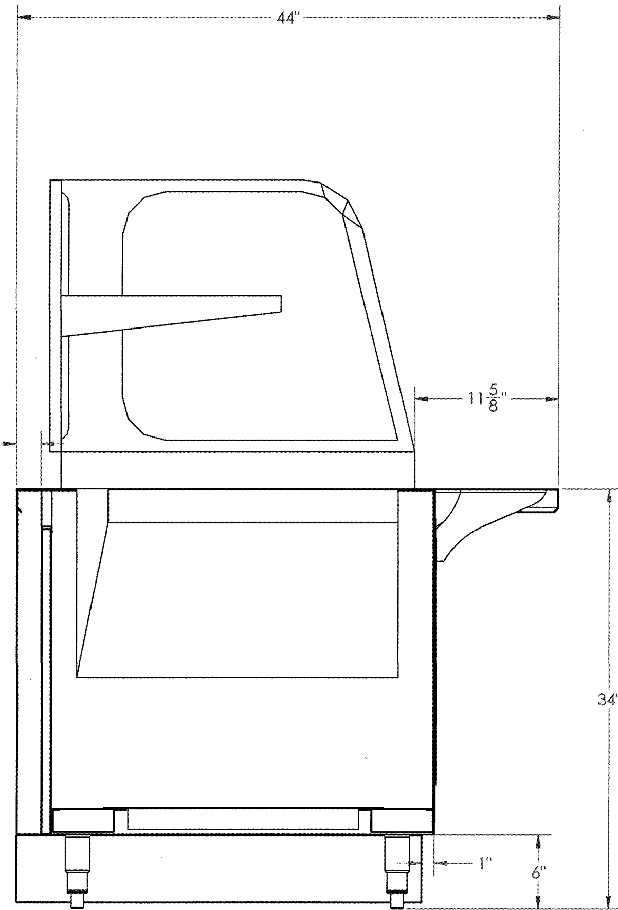
SECTION AT ITEM 3 1 1/2"=1'-0"
